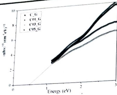
Fig3(b). Indirect band gap of irradiated C series.
