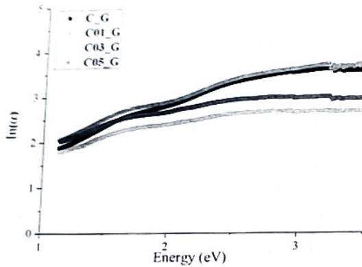
Fig.4. Urbach energy of irradiated C series.
