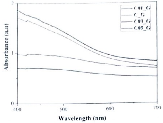
Fig2. Absorption spectra of gamma irradiated glasses.
